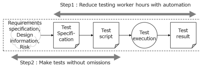
Figure 2 Two steps to promote system test automation
