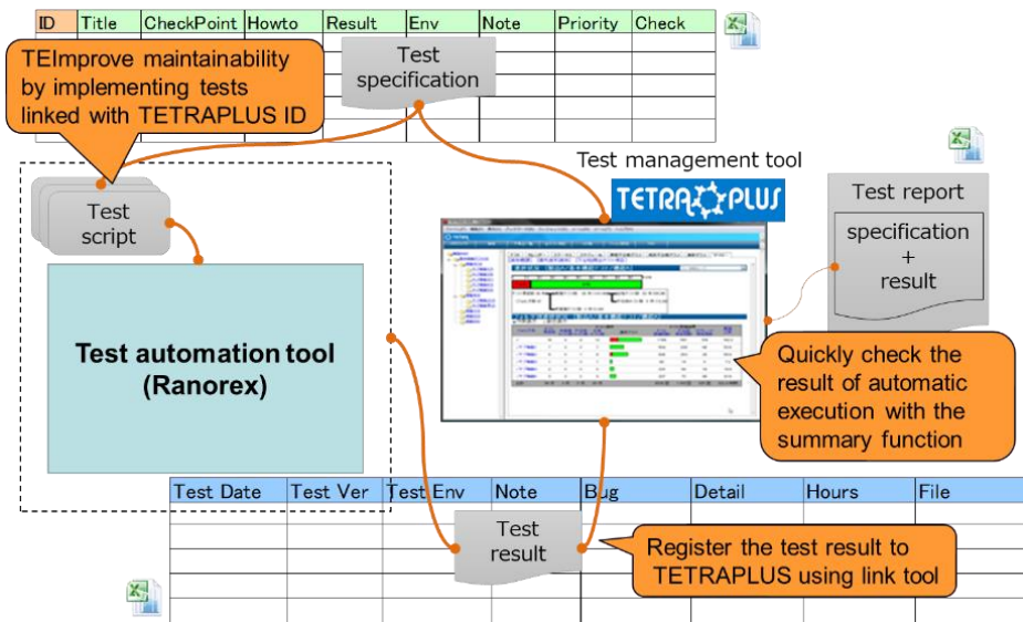
Figure 6 Established system test automation environment
